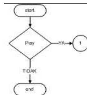
Gambar 5. Flowchart program.bmp
