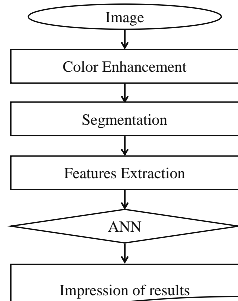
Fig. 1: Processing algorithm
