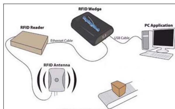
Fig. 7- Communication equipment
