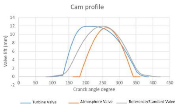
Fig. 2: Came profile
