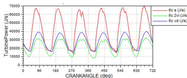
Fig. 4: Power at the turbine
