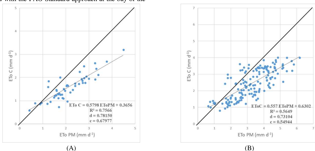
Fig.4: Confrontation between reference evapotranspiration estimated by the classical Penman-Monteith approach ( ET_{oPM} ) and potential demand calculated by the Camargo method ( ET_{oC} ) for the period comprised between March 27, 2008 and August 22, 2011 at Ponta Grossa (A), and between August 26, 2011 and October 14, 2013 at Arapoti (B), PR, Brazil (averages of a 5-day period).
