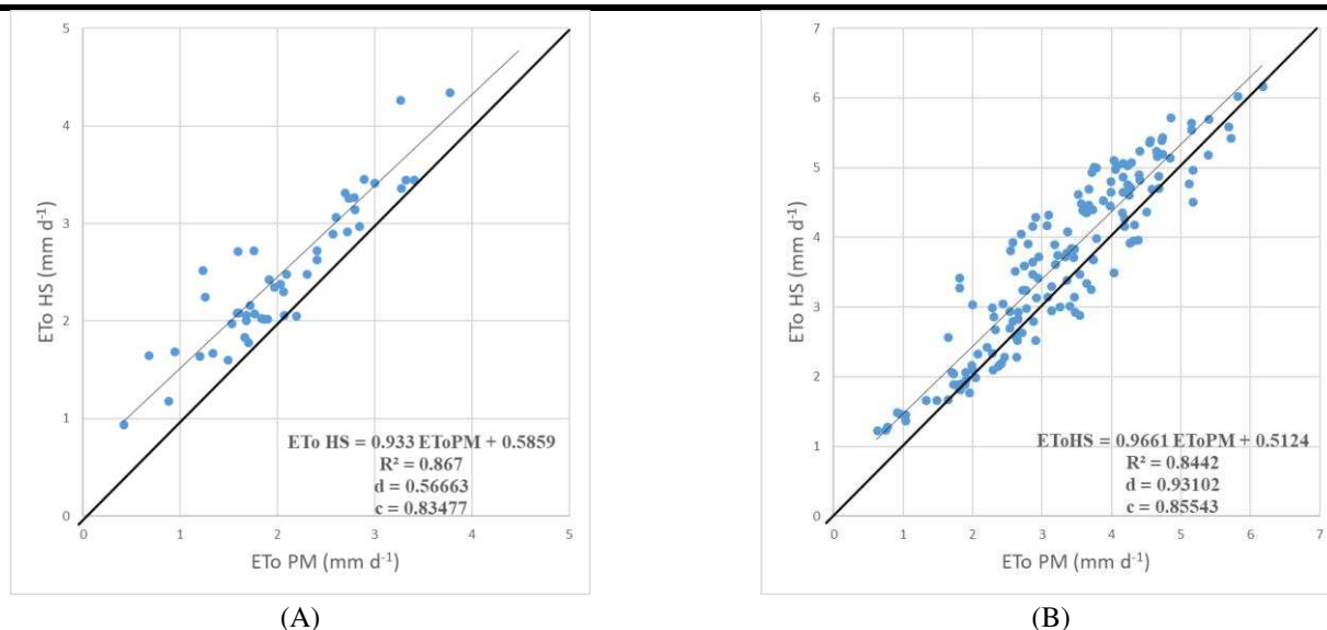
Fig.3: Confrontation between reference evapotranspiration estimated by the classical Penman-Monteith approach ( ET_{oPM} ) and potential demand calculated by the Hargreaves-Samani method ( ET_{oHS} ) for the period comprised between March 27, 2008 and August 22, 2011 at Ponta Grossa (A), and between August 26, 2011 and October 14, 2013 at Arapoti (B), PR, Brazil (averages of a 5-day period).
