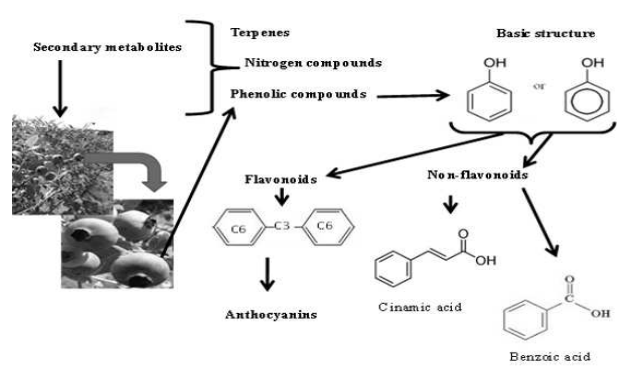
Figure 1: Origin and basic structure of the phenolic compounds in the blueberry
