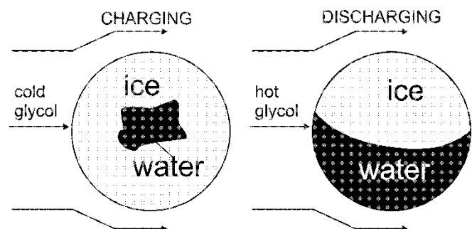
Figure 1 Schema of ice creation in capsule during charging and discharging LHS process.
