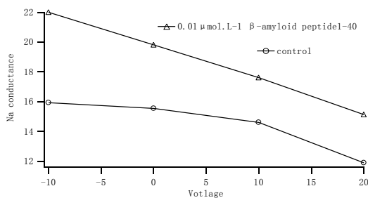
Fig 2. shows the join 0.01\mu\text{mol.L}^{-1} \beta -amyloid peptide 1-40 before and after the effect of intensify voltage and maximum \text{Na}^+ conductivity.
