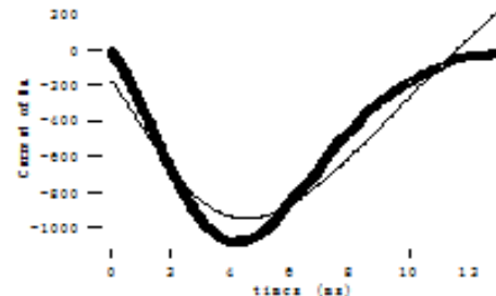
Fig4 shows the join 0.01\mu\text{mol.L}^{-1} \beta -amyloid peptide 1-40 , \text{Na}^+ current changing with time curve
