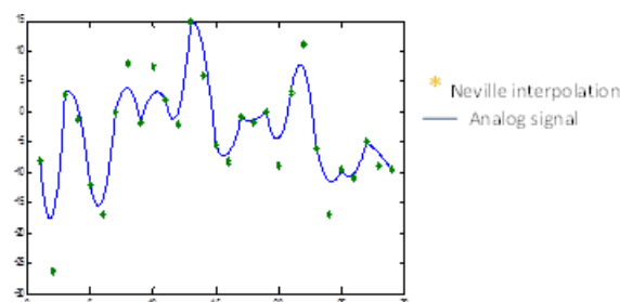
Fig.3: Neville interpolation
