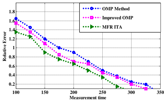
Fig. 4: Errors Behaviour of Reconstruction.
