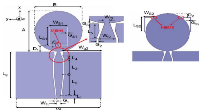
Figure 8: A reconfigurable antenna schematic U-slot and L-stub.
