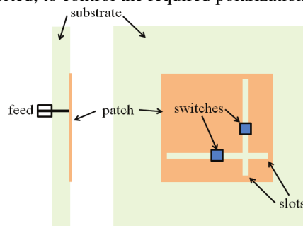
Figure 1: A reconfigurable slotted microstrip patch antenna.
