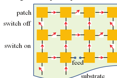
Figure 2: Reconfigurable array antenna patches.
