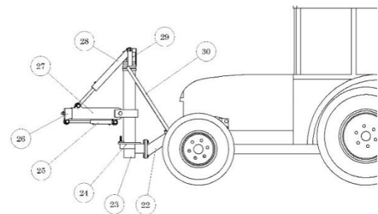
Fig. 3. Platform for support and positioning
