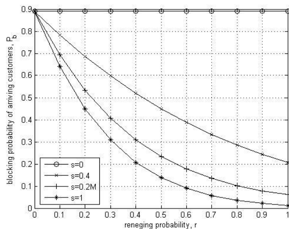
Figure 2. Blocking probability of arriving customers
