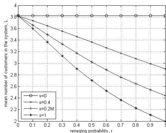
Figure 1. Mean number of customers in the system
