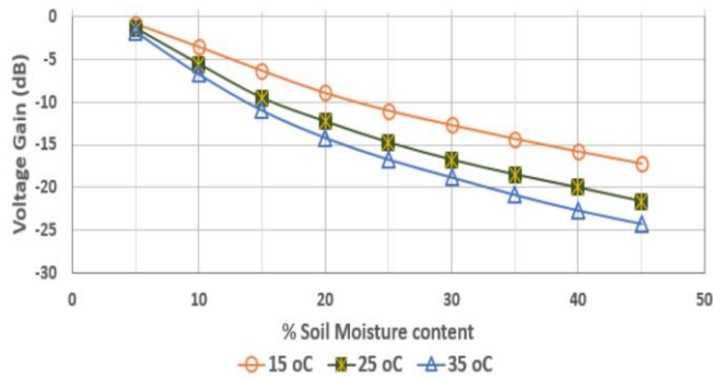
Fig. 3. Attenuation of the applied voltage ( 20 \log \Re\{V_m(t)/(A_0 \sin(\omega t))\} ). Sensor response shown for different soil moisture concentration (5% to 45%) and different temperatures (15 °C, 25 °C and 35 °C).
