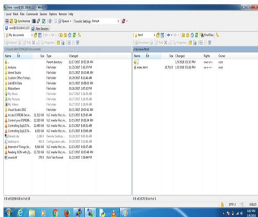
Fig.5: WinSCP software
