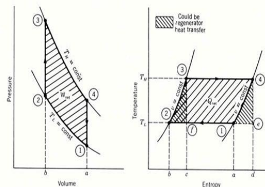
Ideal Pressure-Volume and Temperature-entropy charts of the Stirling cycle.
