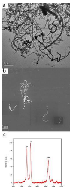
Fig.2. Characterization data for MWCNTs. (a) TEM image; (b) SEM image; (c) Raman spectrum.
