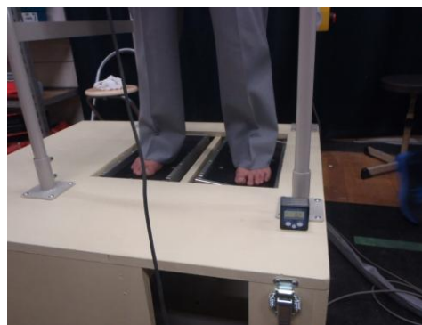
Figure. 2 Standing position on the motion-driven foot plate during movements of the ankle joints.
