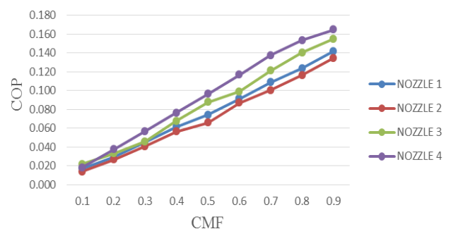
Fig.5: Variation of COP vs. CMF at \theta = 30^\circ
