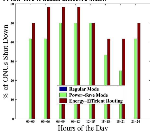
Fig. 3. Power savings in energy-aware WOBAN.
