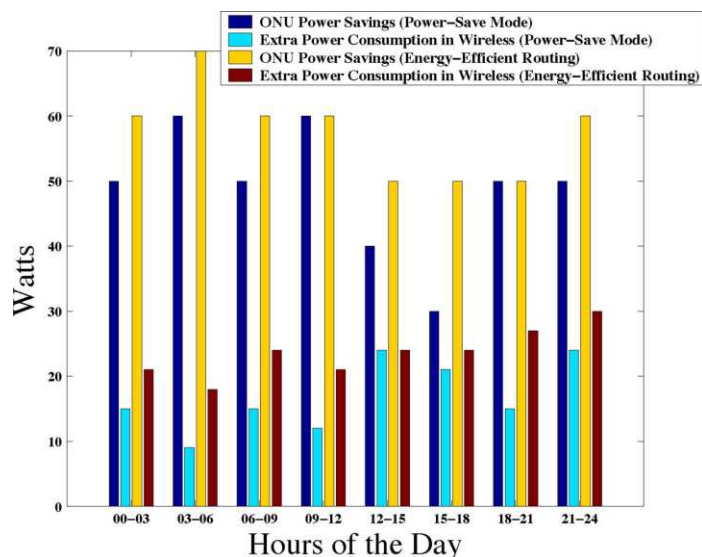
Fig. 4. Power savings versus extra wireless power.
