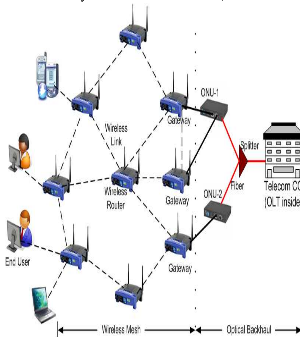
Fig. 1. WOBAN architecture
