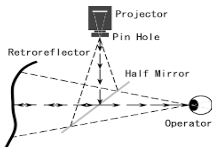
Fig 3:- RPT Principle
