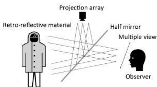
Fig 5:-Phased Array Optics
