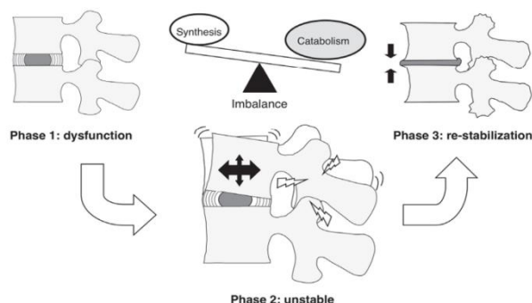
Figure20: Schematic sketch of degeneration of intervertebral disc, loses of water content by increases of catabolism (Phase 1), movement and load on damaged disc (Phase 2), failure or reconstruction of IVD (Phase 3) (Adapted from The potential role of mesenchymal stem cell therapy for intervertebral disc degeneration, Frank Acosta, et al ).
