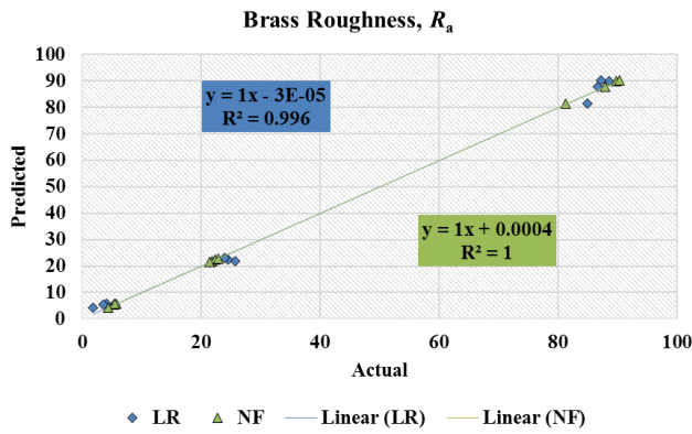
Figure 8: Brass roughness prediction model with linear regression
