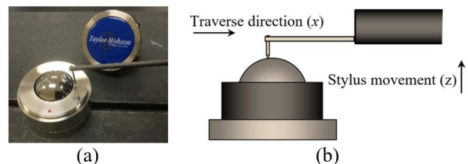
Figure 4: (a) image of standard calibration ball radius D = 22.0161 \text{ mm} , 112/1844, Serial No. 639-506-B (b) ball with nominal 2 \mu\text{m} stylus
