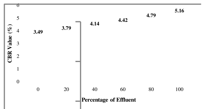
Fig.4. CBR Value Vs Percentage of effluent
