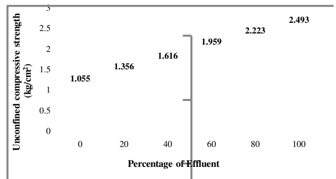
Fig.3. Unconfined Compressive Strength
