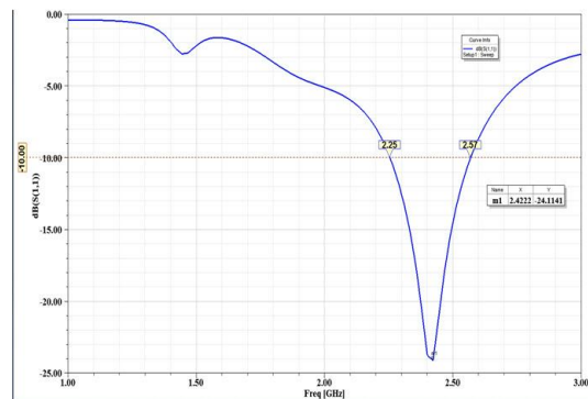
Figure 4 shows the s11 parameter of the microstrip antenna.
