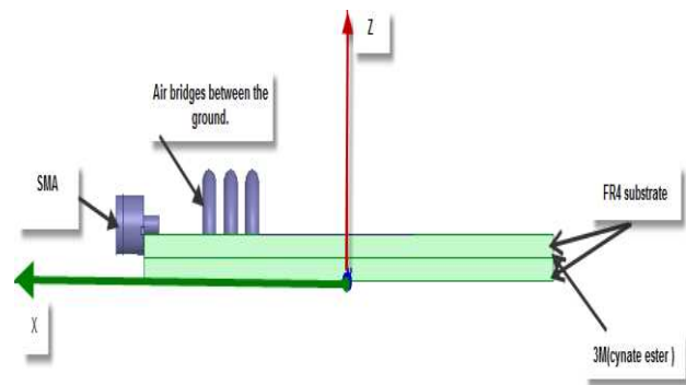
Figure 3 Shows the side view of designed antenna in HFSS Software.
