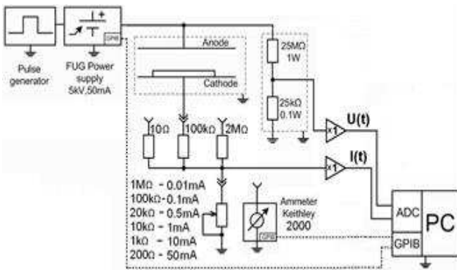
Figure 4: Block diagram of the electric circuit of the IMLS in diode configuration [48].
