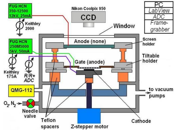
Figure 5: Triode (diode) configurations of the IMLS [48].
