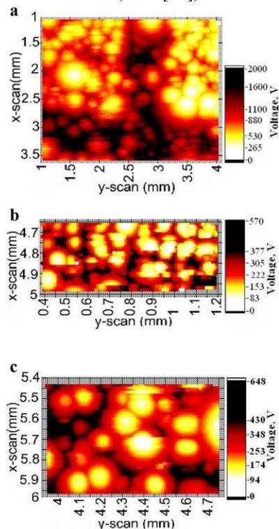
Figure 19: (Color online) Regulated voltage maps (for 1 nA current) of FECs on a chip with structured CNT arrays having 50 \mu\text{m} diameter pillars: (a) two upper quadrants corresponding to Figure 15 (scanned area 7.5 \text{ mm}^2 , low resolution anode \varnothing 30 \mu\text{m} , gap 60 \mu\text{m} ); (b) lower left ( 0.28 \text{ mm}^2 ); (c) lower right quadrant ( 0.64 \text{ mm}^2 ) in high resolution (anode \varnothing 3 \mu\text{m} , gap 15 \mu\text{m} ).
