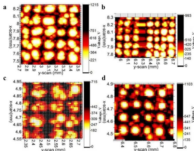
Figure 18: (Color online) Medium resolution regulated voltage maps (for 1 nA current, anode \varnothing 8 \mu\text{m} ,
