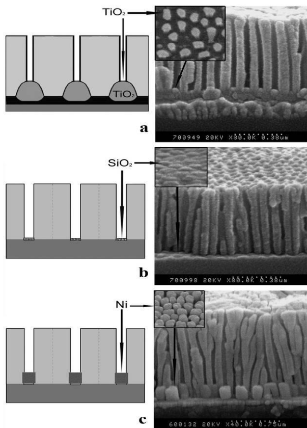
Figure 24: Three different CNT contact interfaces: (a) \text{Si}/\text{Ti}/\text{TiO}_2 (type 1); (b) \text{Si}/\text{SiO}_2 (type 2); (c) \text{Si}/\text{SiO}_2/\text{Ni} (type 3).
