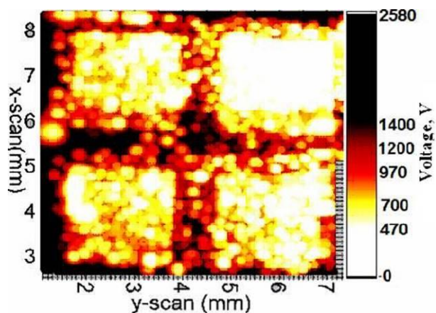
Figure 17: (Color online) Regulated voltage map for 1 nA current FECs on a chip with structured CNT arrays having 20 \mu\text{m} diameter pillars (scanned area 36 \text{ mm}^2 , low resolution anode with the diameter \varnothing 30 \mu\text{m} , cathode-anode gap 40 \mu\text{m} ).
