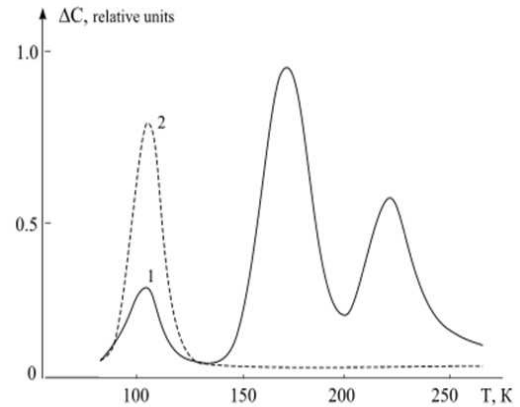
Fig.2. Typical DLTS spectra of the samples n-Si<V> - curve 1 control samples (heat-treated n-Si) - curve 2.
