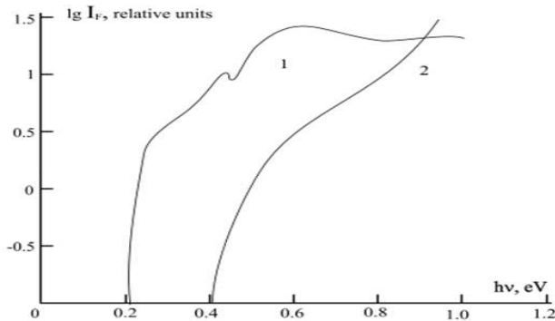
Fig. 1. Normalized to a constant stream of quanta spectra of photoconductivity
