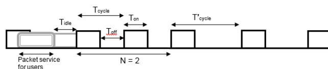
Figure 5: Parameters for dynamic cell deactivation
