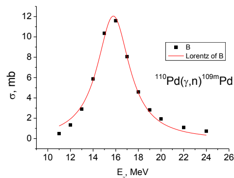
Fig.3. The reaction cross section is ^{110}\text{Pd}(\gamma, n)^{109\text{m}}\text{Pd} (TALYS-1.6).
