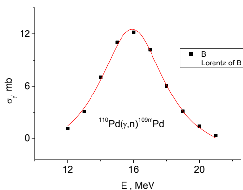
Fig.2. The reaction cross section is ^{110}\text{Pd}(\gamma, n)^{109\text{m}}\text{Pd}
