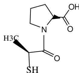
Figure 3. Chemical structure of captopril
