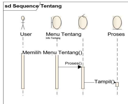
Gambar 10. Sequence Diagram Menu Tentang
