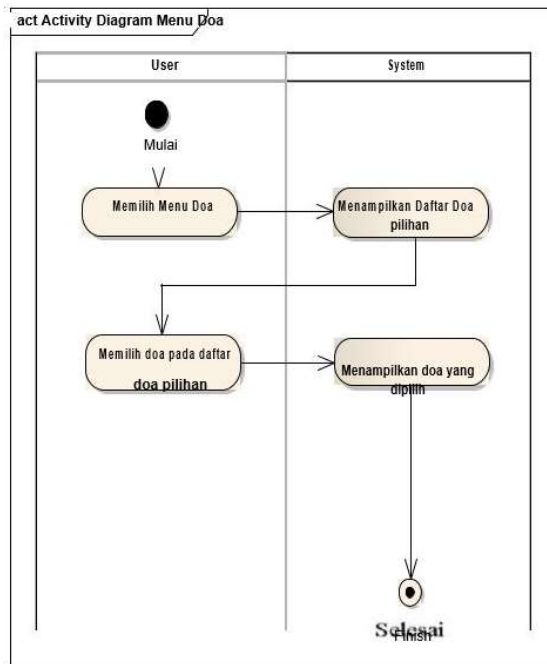
Gambar 4. Activity Diagram Menu Doa-Doa
