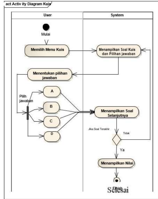
Gambar 5. Activity Diagram Menu Kuis
