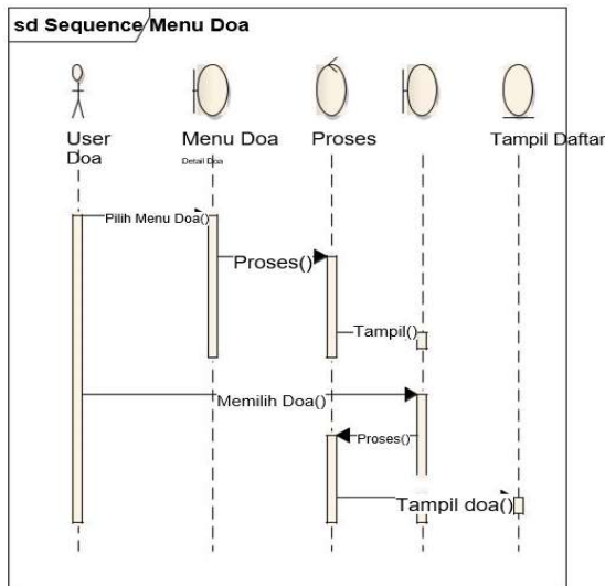
Gambar 8. Sequence Diagram Menu Doa
