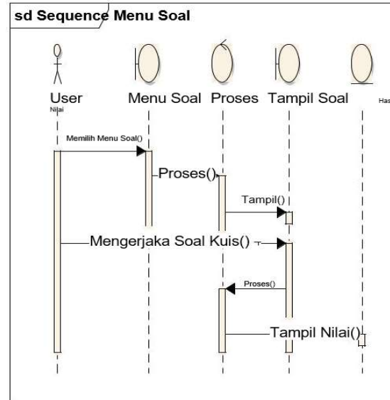
Gambar 9. Sequence Diagram Menu Kuis
