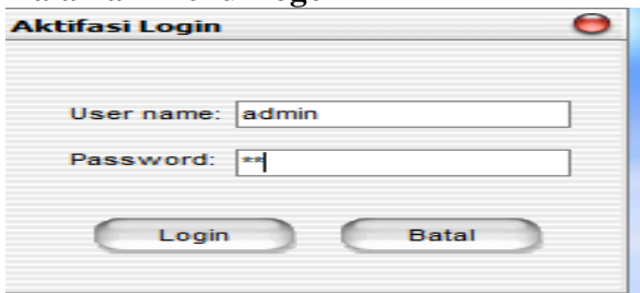
Gambar 5. Menu Logon
