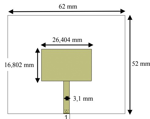
Gambar 3. Antena mikrostrip rectangular \frac{1}{4} lamda
