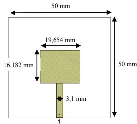
Gambar 1. Antena mikrostrip rectangular awal
