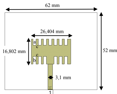
Gambar 6. Antena mikrostrip rectangular gerigi
