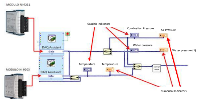
Fig. 11: DAQ assistant.
