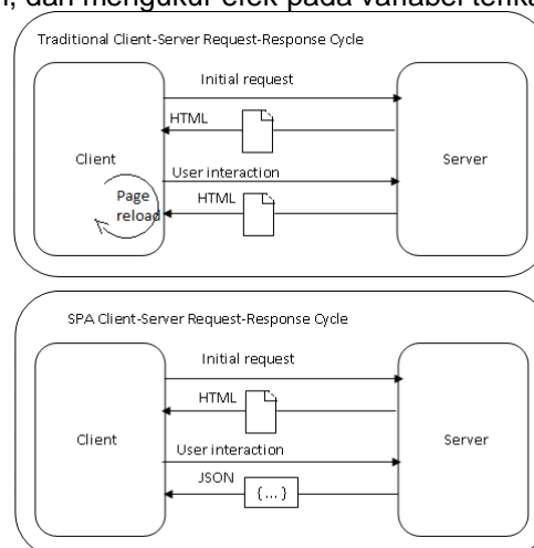
Gambar 2. Client-Server Request-Response Cycle
