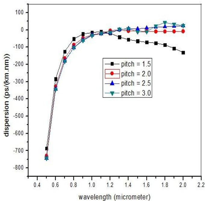
Figure: 10. Comparison of chromatic dispersion of proposed Honeycomb PCF when air hole diameter is 1.0\mu\text{m} .
