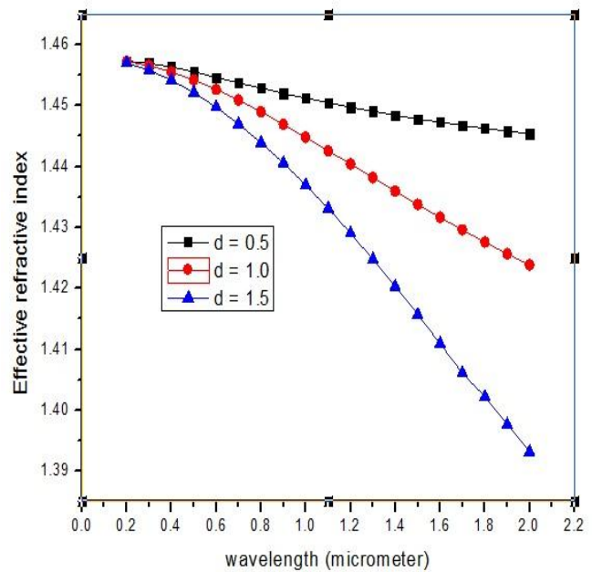
Figure: 6. Comparison of Effective refractive index for constant Pitch (Pitch = 2.0 \mu\text{m} )
