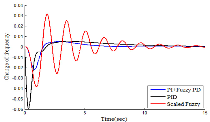
Figure 9: Frequency deviations of 1% load changes
