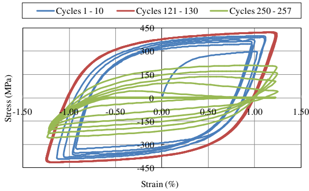
Fig. 7 Typical stress-strain hysteresis curves for \pm 1.25\% strain amplitude
