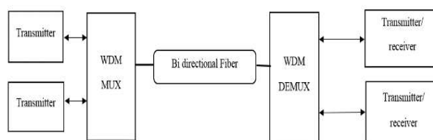
Fig 1. Block diagram of bi-directional wdm-pon
