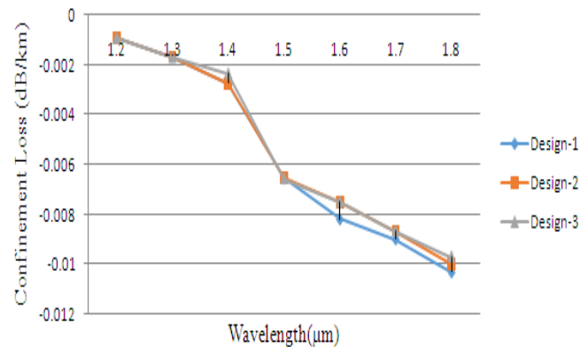
Fig. 7 Comparison of Confinement Loss for Design-1 to Design-3
