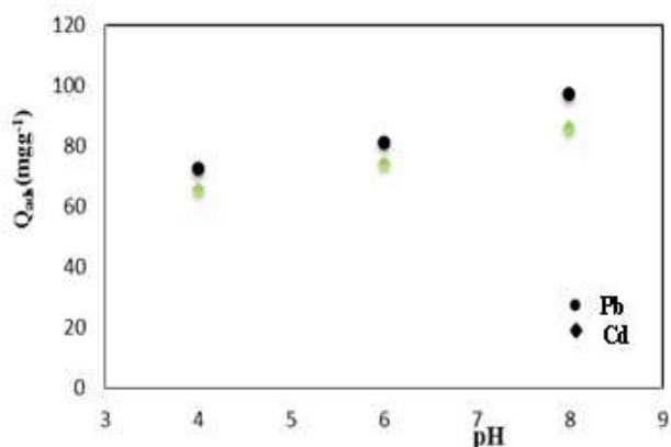
fig.8: Effect of pH on cadmium and lead removal by Na saturated bentonite ( [metal] = 10^{-4} M, T = 20 °C)
