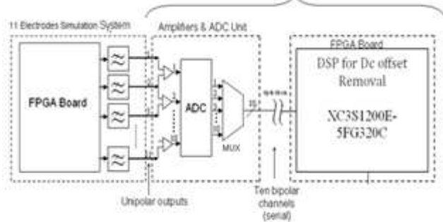
Fig. III. Block diagram of the complete system.
