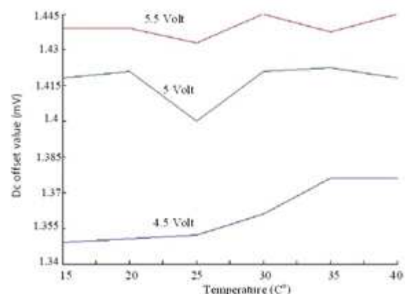
Fig.6.The DC offset variation curve for delay and add channel
