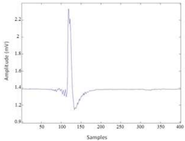
Fig.6. The DC offset value for the delay and add channel before removing the DC offset.
