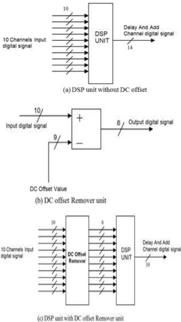
Fig. 7. DSP unit with and without DC offset Remover
