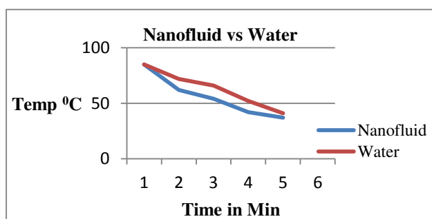
Fig02.Nanofluid vs Water
