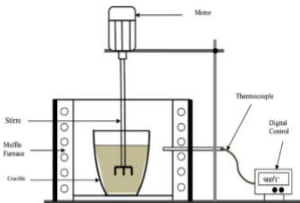
Figure 2. Schematic view of setup for stir casting (color figure available online).
