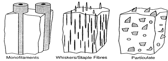
Figure 1. Schematic presentation of various types of metal matrix composites [4].
