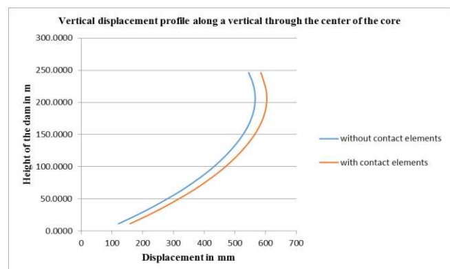
Figure 4: Vertical displacement profile along vertical
