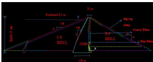
Fig. 1 Cross-section of Dam
