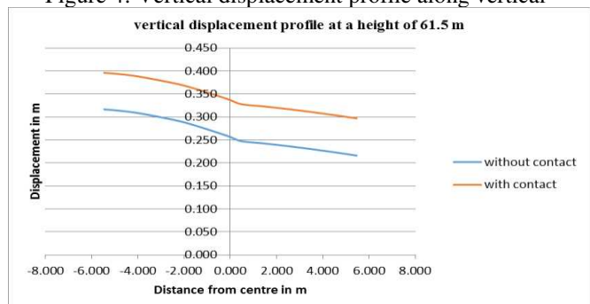
Figure 5: Vertical displacement profile along horizontal
