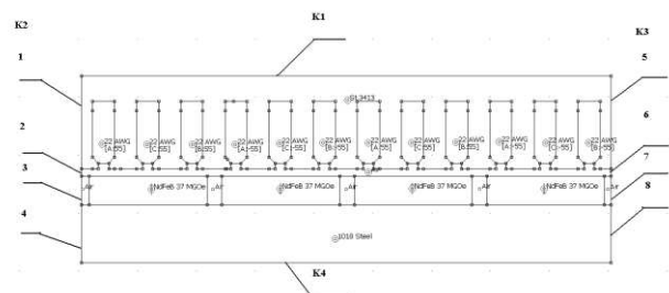
Fig. 8. The FEMM model of PMLSM with PMs
