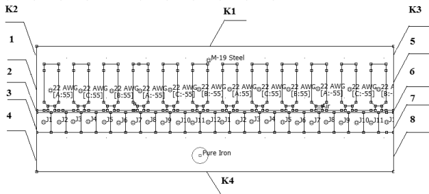
Fig. 3. FEMM model of linear synchronous servomotor
