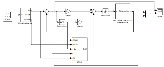
Figure 6: Simulation system
