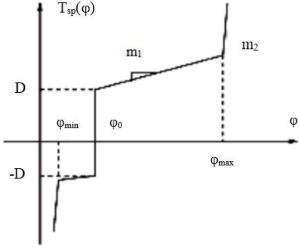
Figure 3. Nonlinear Spring
