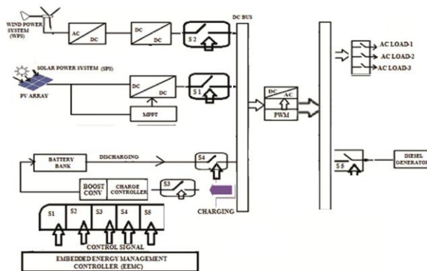
Figure10. Block diagram of mode 5
