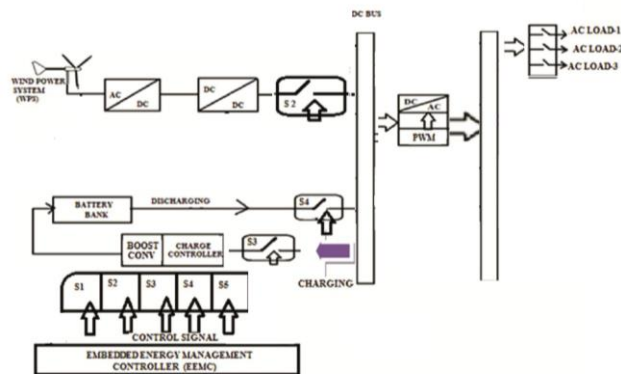
Fig9. Block diagram of mode 4
