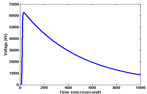
Figure 11: Curves surges simultaneously on the three phase conductors according to Heidler function
