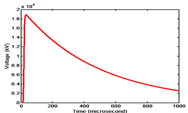
Figure 6: Curve of surge on the n^01 conductor struck down.
