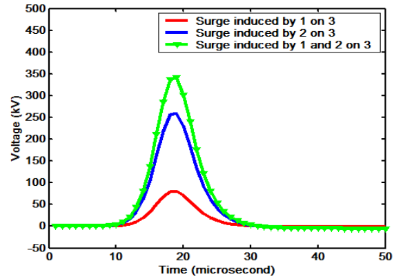
Figure 10: Curves of surges induced simultaneously by n^01 and n^02 conductors according to the function of Heidler.
