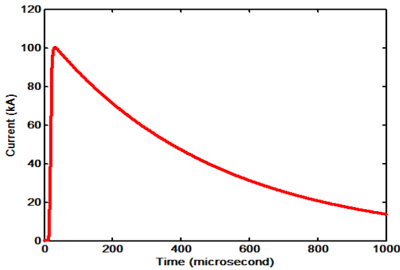
Figure 3: Wave current of lightning according to the function of Heidler.
