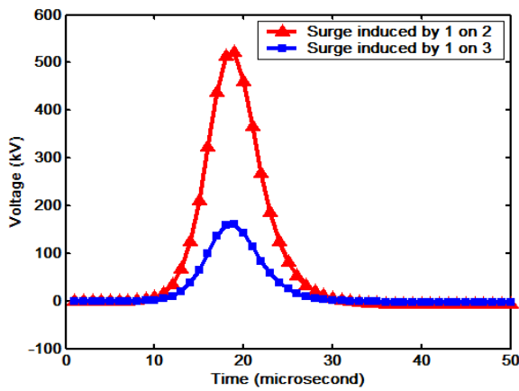
Figure 8: Curve of induced surges on the n^02 and n^03 conductors according to the function of Heidler
