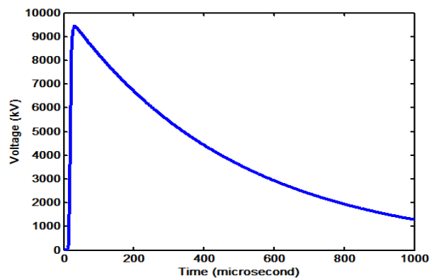
Figure 9: Curve of the surge on the n^01 and n^02 conductors according to the function of Heidler
