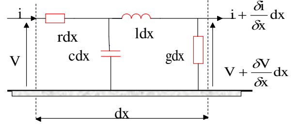
Figure 4: Diagram of a high voltage line
