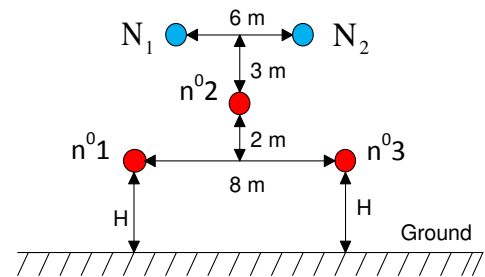
Figure 1: Configuring of Ngo -Brazzaville line
