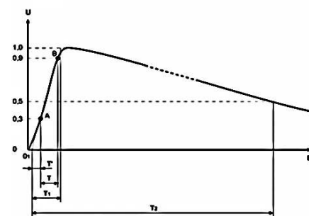
Figure 2: Example of the wave of standardized lightning ( 1,2/50 \mu s ) by IEC 60 with T_1 = 1,2 \mu s and T_2 = 50 \mu s
