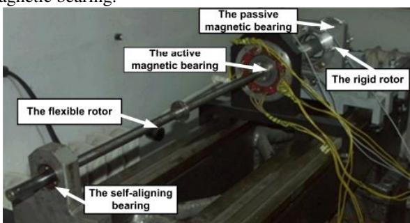
Fig 4: The lab stand for experimental tests of PMB
