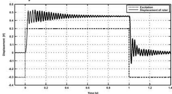
Fig 9: The step response of the PMB
