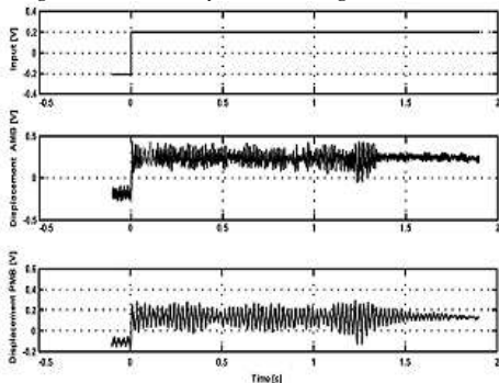
Fig 8: Step response of active (AMB) and passive (PMB) magnetic bearing to excitation by external signal at the axis Oy.
