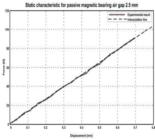
Fig 6: The static characteristic of passive magnetic bearing
