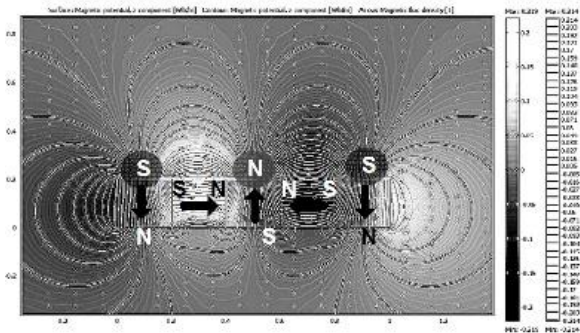
Fig. 3. Configuration of magnets in Halbach array.
