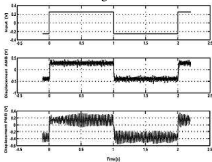
Fig 7: Step response of active (AMB) and passive (PMB) magnetic bearing to excitation by external signal at the axis Ox
