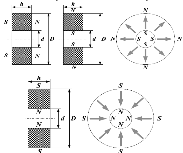
Fig 1: Ring-shaped magnets with radial and axial orientation of magnetization.
